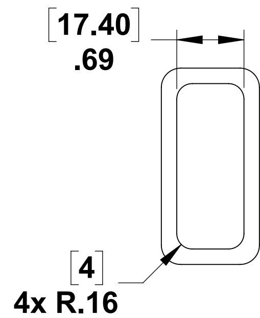
ADJUSTABLE CONNECTOR-1
