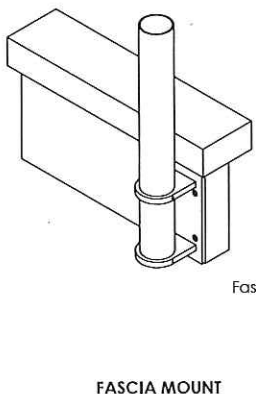
FASCIA MOUNT
