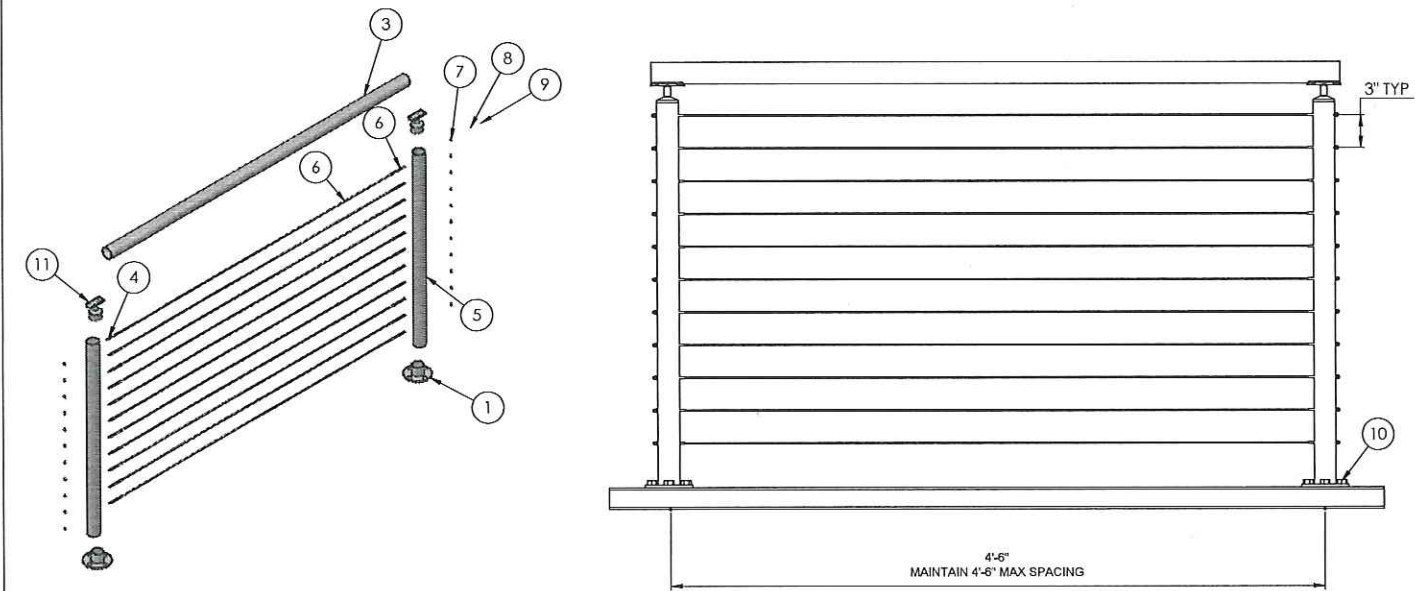
LEVEL 36" STANDARD GUARD RAILING
