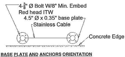
BASE PLATE AND ANCHORS ORIENTATION
