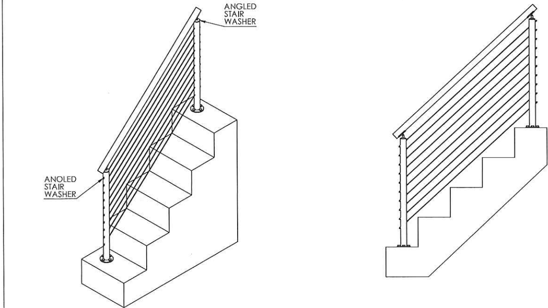
STAIRS 36" STANDARD GUARD RAILING
