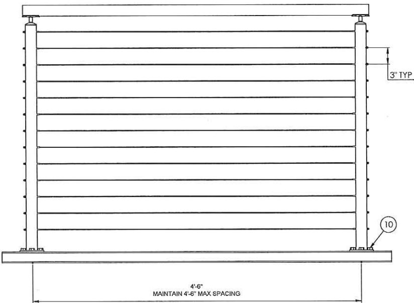
LEVEL 42" STANDARD GUARD RAILING
