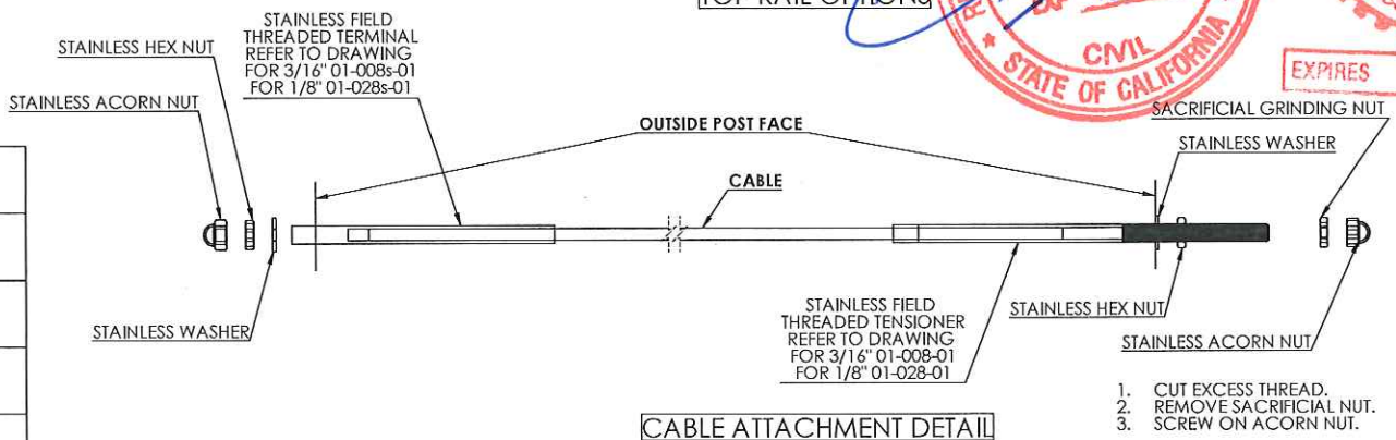
CABLE ATTACHMENT DETAIL
