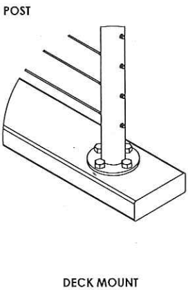
DECK MOUNT
