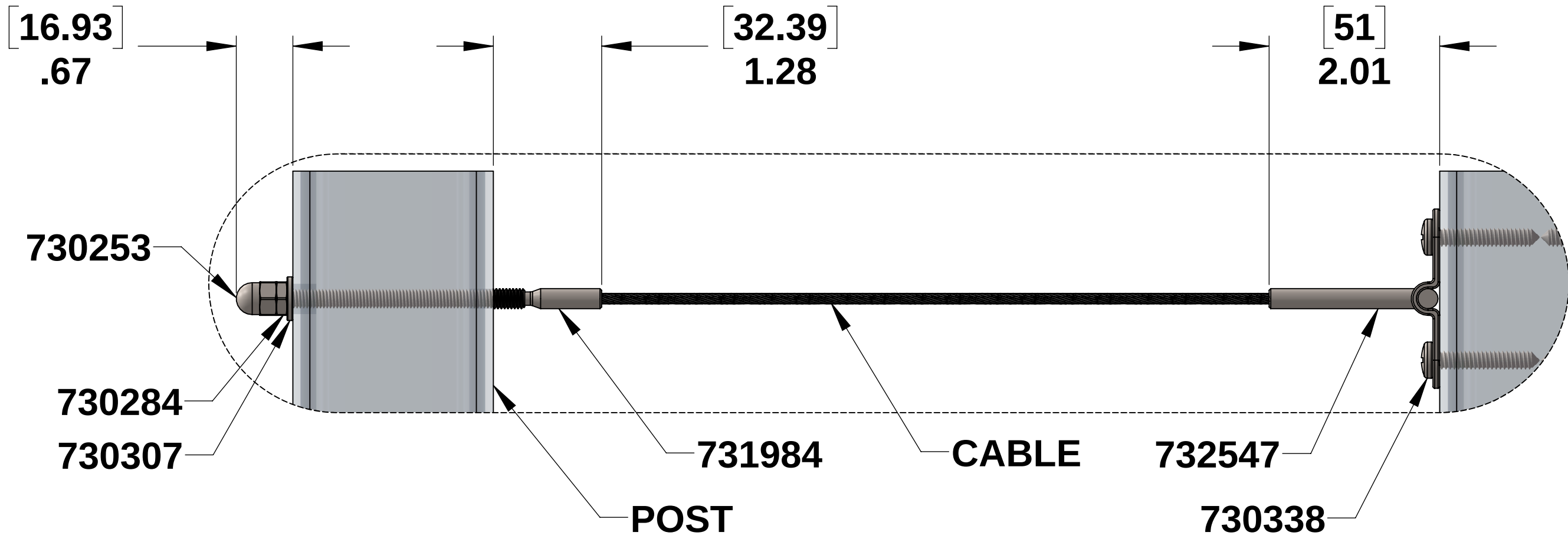
DETAIL B OPTION #1A
