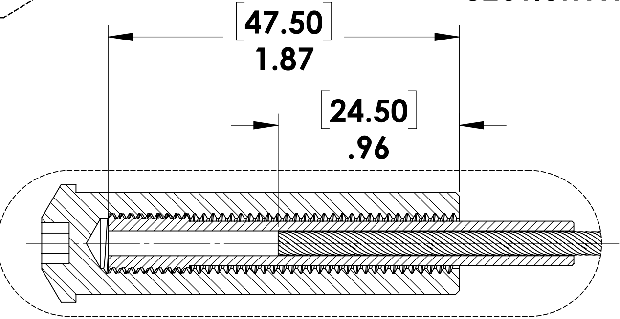
DETAIL B SCALE 2 : 1
