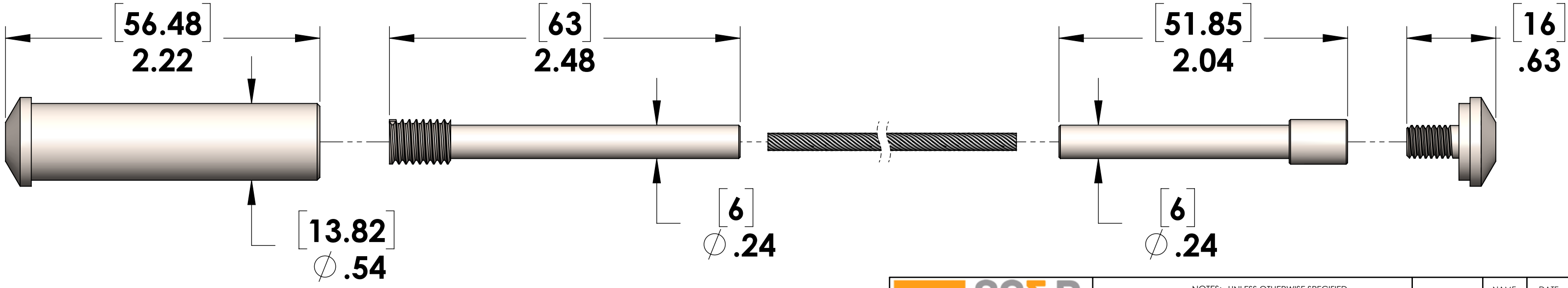
DETAIL B SCALE 2 : 1
