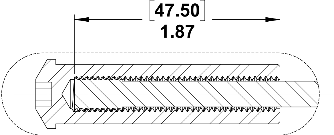
DETAIL B SCALE 2 : 1
